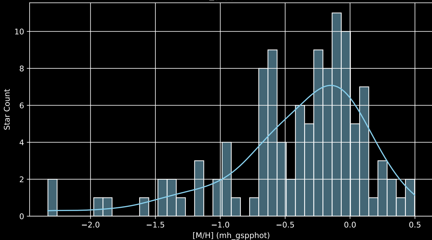
APOGEE DR17 Field: [016+02 [M/H] (mh_gspphot) (n= 114)
