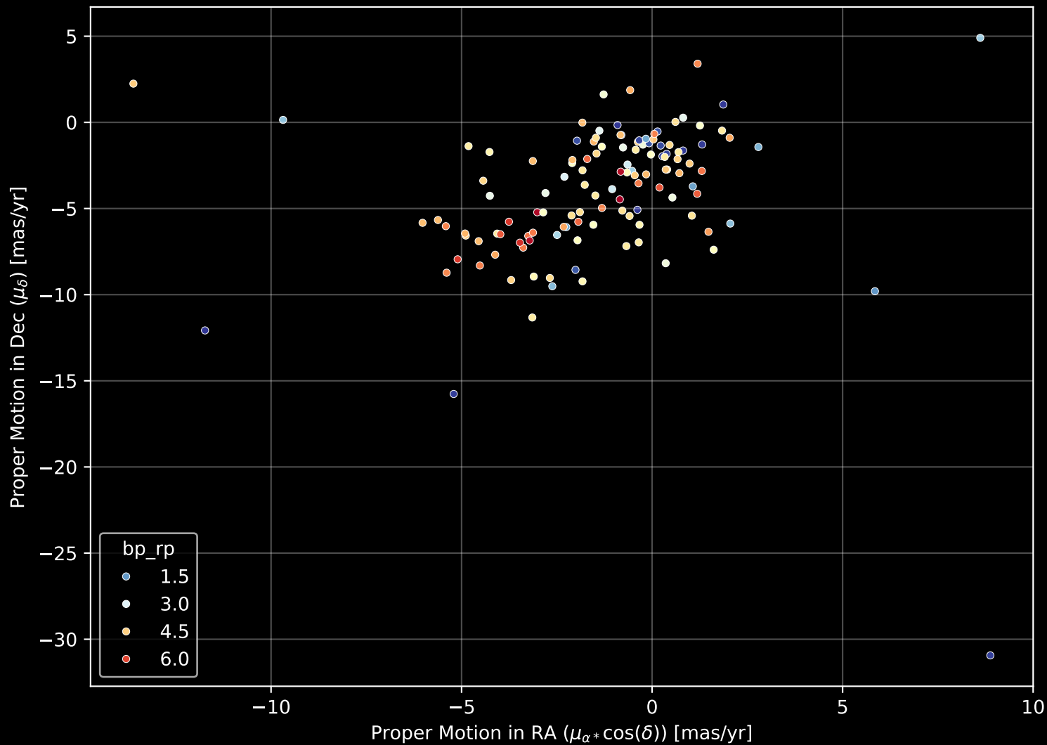
APOGEE DR17 Field: [016+02] Proper Motion Diagram (n= 125)
