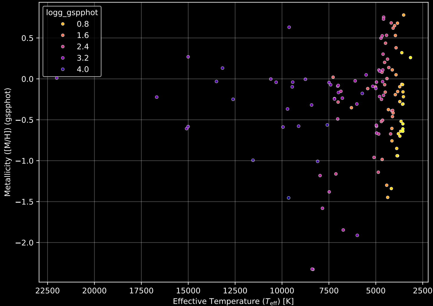
APOGEE DR17 Field: [016+02] Stellar Population Parameters (n= 125)
