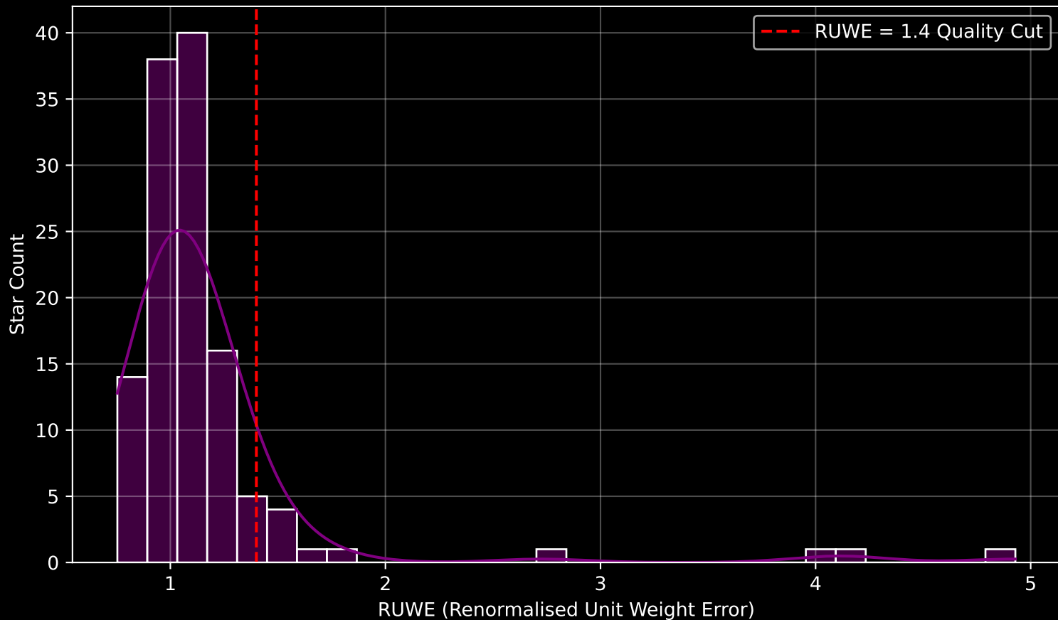
GAPOGEE DR17 Field [016+02] RUWE Distribution (n= 123)
