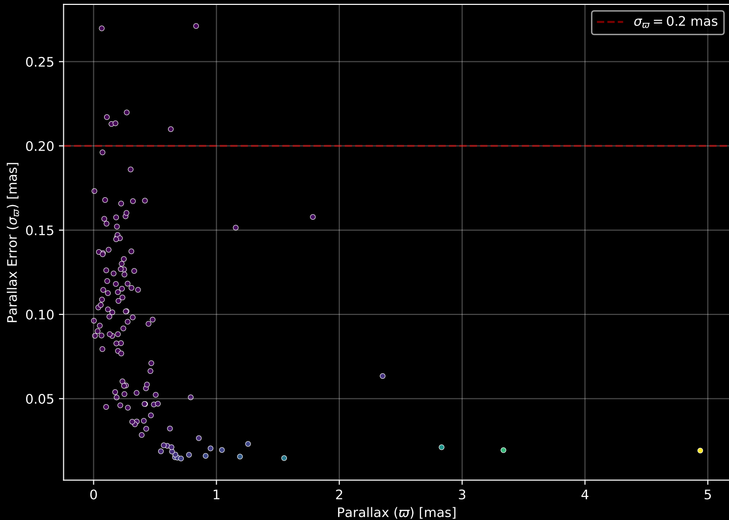
APOGEE DR17 Field: [016+02] Parallax Quality (n= 125)
