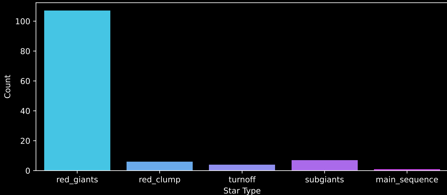
APOGEE DR17 Field: [016+02] Count plot of Star Type
